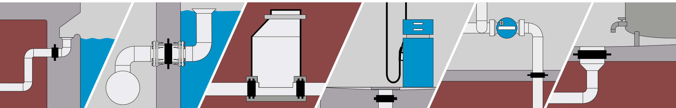
Swimming pool drain pipes in walls and foundation plates
